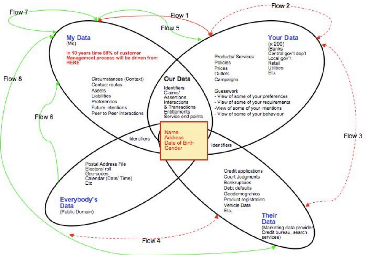
Figure 2: Data Relationships
