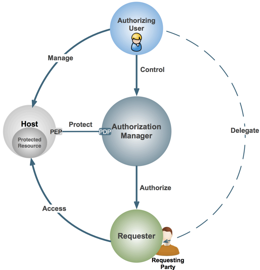
Figure 7: User-Managed Access
